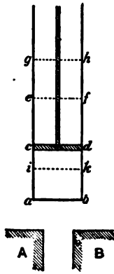
FIG. 4. Carnot's Cylinder.
