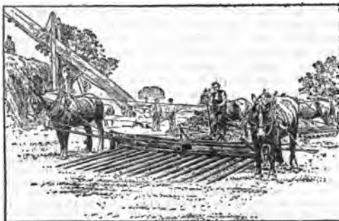
FIG. 5.—Sweep Rake.
