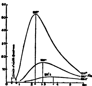
FIG. 7.—Distribution of energy in the spectrum of a black body.
