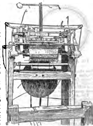
FIG. 3.—Hand Stocking Frame.
