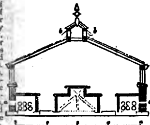
FIG. 4.—Section of Plant Stove.
