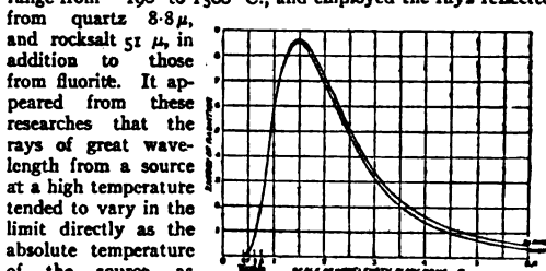
FIG. 8.—Distribution of energy in the spectrum of full radiation at 2000° Abs. according to formulae of Planck & Wien.
