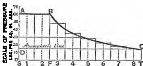
Fig. 3.—Watt's Indicator Diagram. Patent of 1782.
