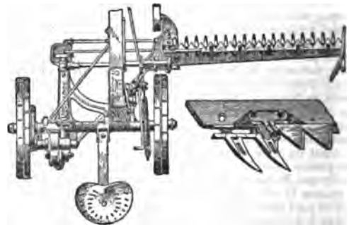
FIG. 1.—Mower (viewed from above) with enlarged detail of Blade. (Harrison, M'Gregor & Co.)
