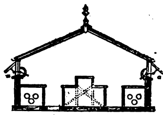
FIG. 3.—Section of Greenhouse.
